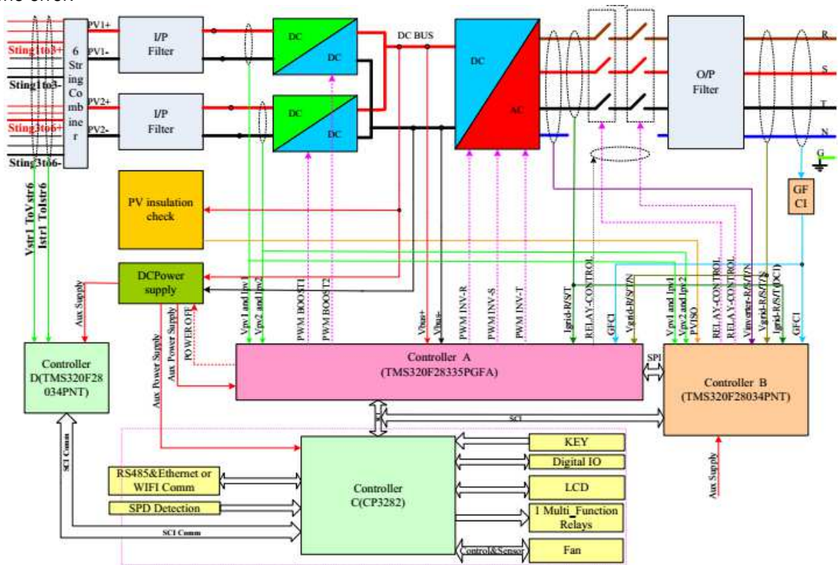
Figure 1-Block diagram
